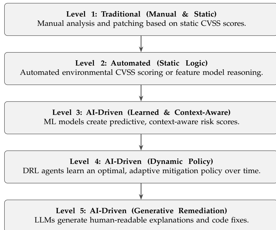
Figure 4. The evolution of vulnerability mitigation strategies identified in this review. The trend progresses from static, manual processes (Level 1), to automated but rigid logic (Level 2; e.g., VMC [13] and AMADEUS-Exploit [41]), and finally to AI-driven systems that are context-aware (Level 3; e.g., VPSS [42] and LICALITY [39]), dynamic (Level 4; e.g., Deep VULMAN [23]), and generative (Level 5; e.g., LLM-based remediation approaches [15,24]).
